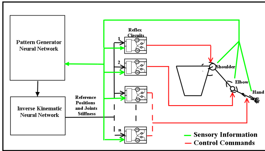
Fig. 2. Control Architecture
