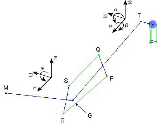
Fig. 5. Arm kinematic
