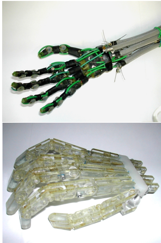
Fig. 1. Blackfingers and WhiteFingers Endoskeleton
